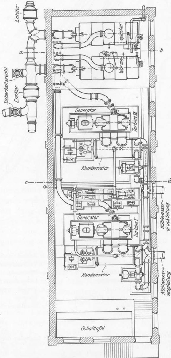
Figur 23, Grundriß.
