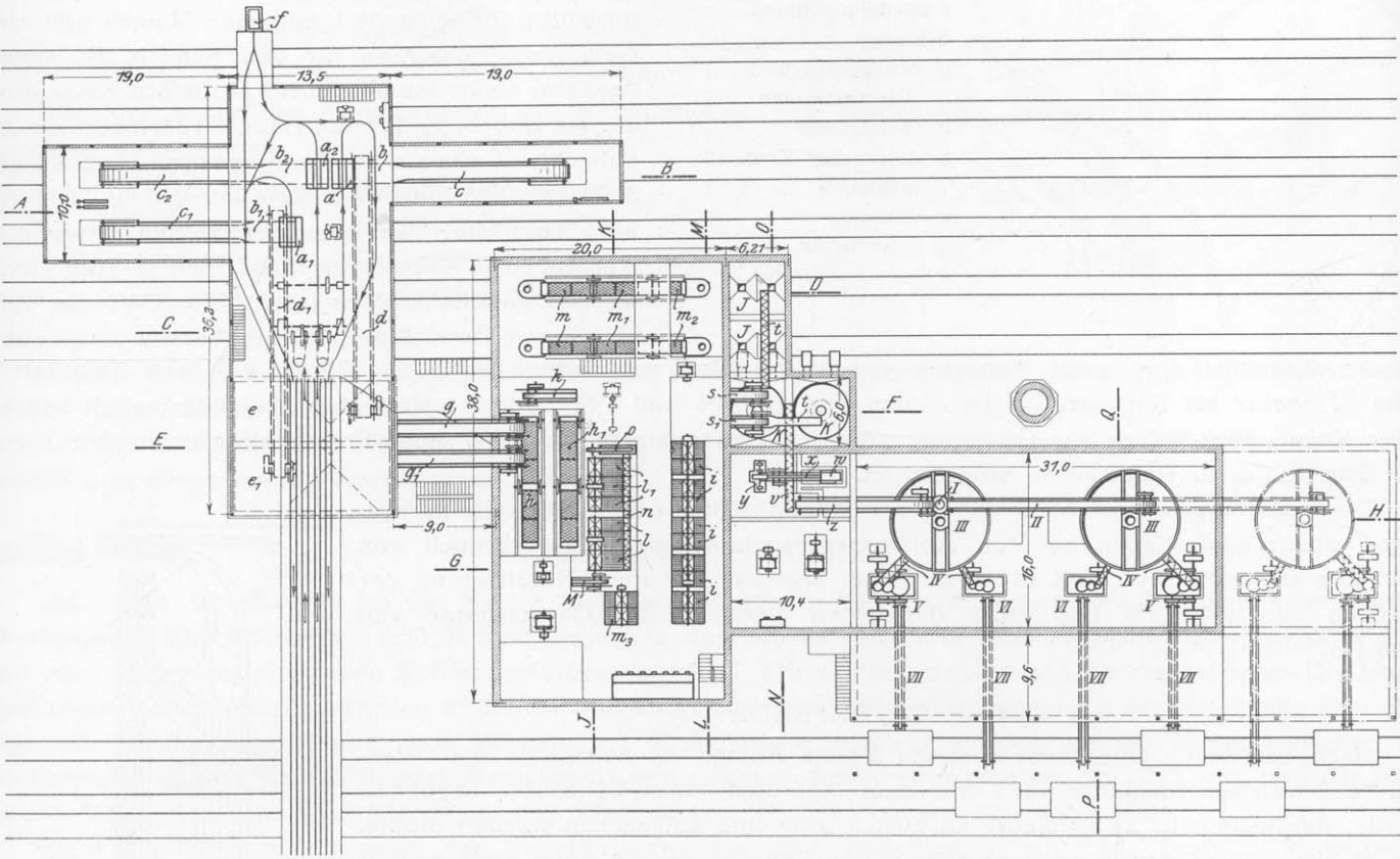
Figur 12: Lageplan
